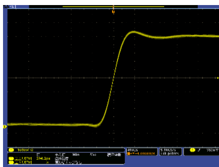
Rise-time 395ps
